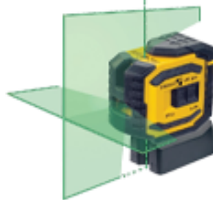
Stabila 03185 LAX300G Green Beam Cross Line Plus Plumb Dots Laser Level
